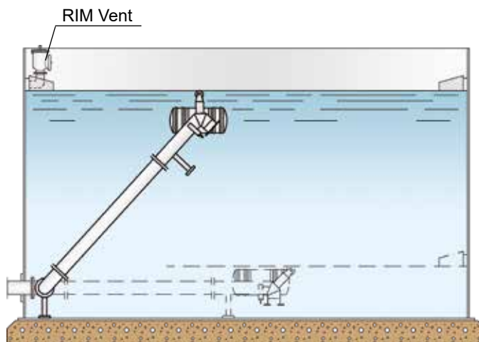
PROTEGO® SA/S for floating roof tanks
