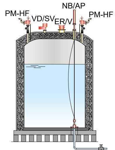
LIN-LOX-LAR Storage Tank
