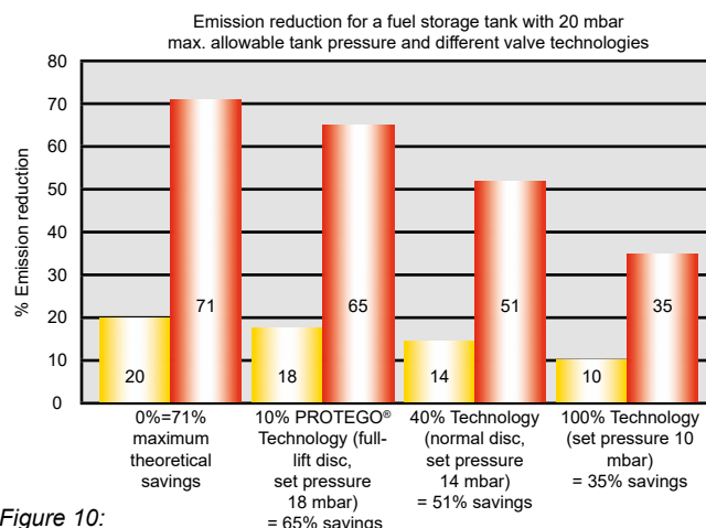
Figure 10: Stored product - fuel: comparison of product savings at different over-pressure levels versus the free vented storage tank: example of product loss at 20 mbar allowable tank pressure savings in % at different overpressure
