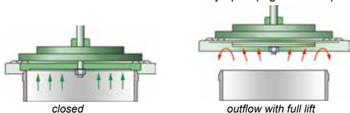
Fig. 1: Outflow with a full-lift pallet and air cushion seal
