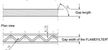
Figure 7: FLAMEFILTER® (a) with gap widths and gap lengths and PROTEGO® flame arrester unit (b) with FLAMEFILTER®, spacer, and FLAMEFILTER® casing
