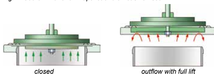
Fig. 2: Outflow with a full-lift pallet and metal seal
